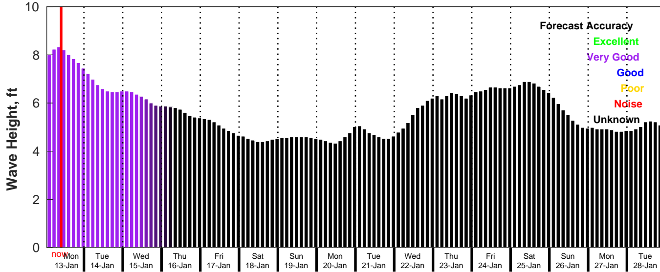
GFS Wave Forecast for NDBC 51209 from 13-Jan-2025 01:00:00 to 29-Jan-2025 01:00:00
