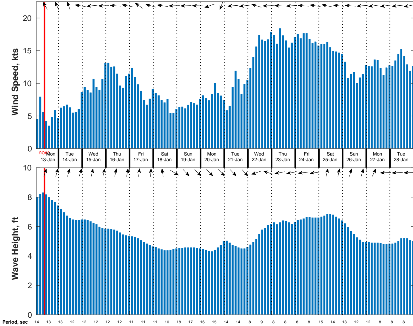
Wind & Wave Forecast for NDBC 51209 from 13-Jan-2025 01:00:00 to 29-Jan-2025 01:00:00
