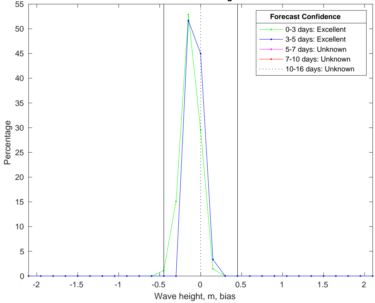
NDBC 52211 vs CMEMSWaves Bias Histogram: 13-Jan-2025
