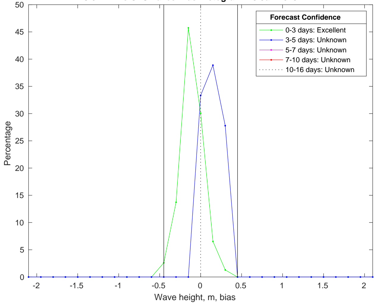
NDBC 52211 vs GFSWaves Bias Histogram: 13-Jan-2025
