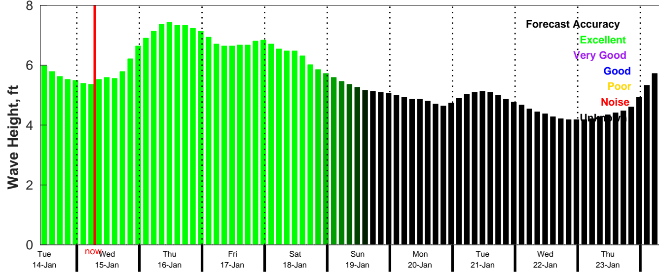
CMEMS Wave Forecast for NDBC 52211 from 13-Jan-2025 10:00:00 to 23-Jan-2025 10:00:00
