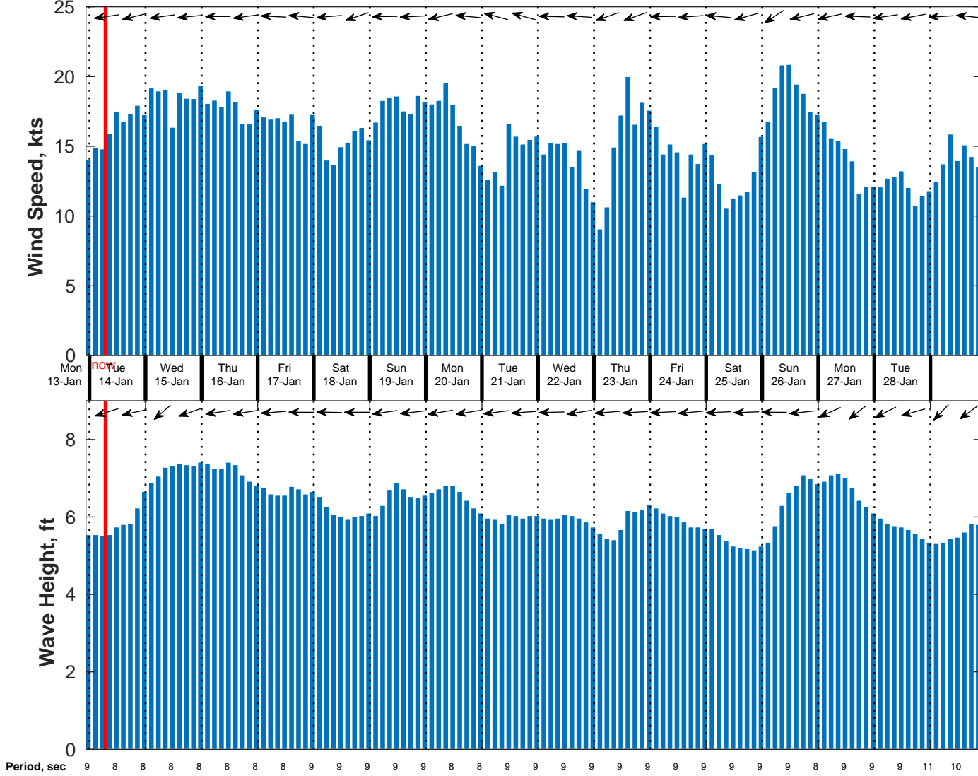
Wind & Wave Forecast for NDBC 52211 from 13-Jan-2025 22:00:00 to 29-Jan-2025 22:00:00
