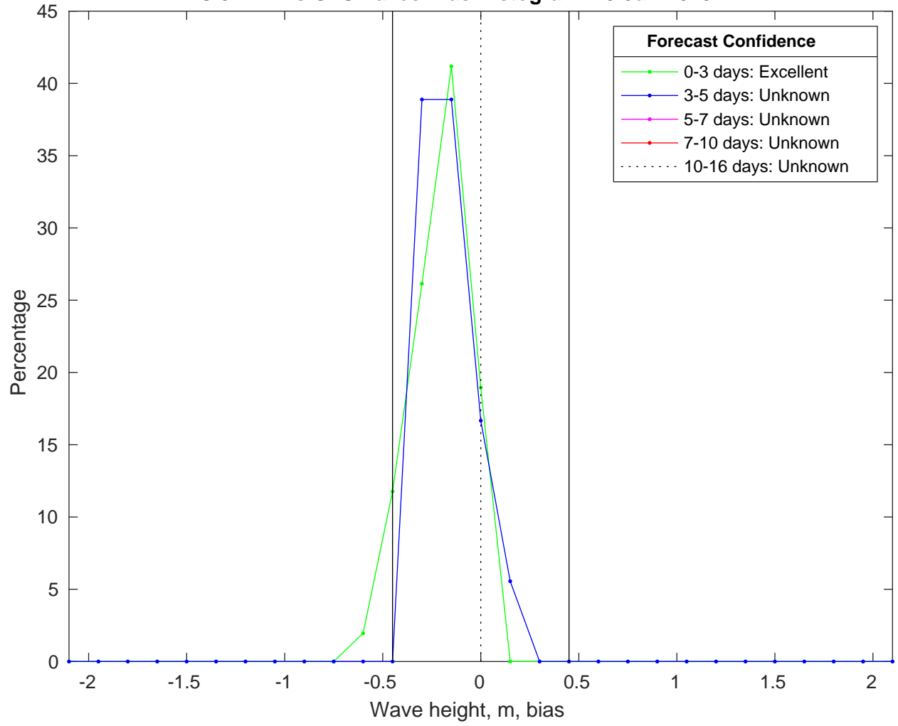
NDBC 52212 vs GFSWaves Bias Histogram: 13-Jan-2025
