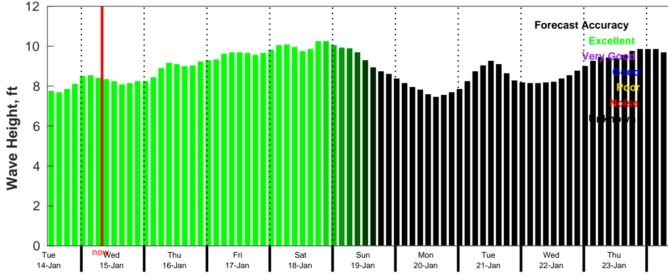
CMEMS Wave Forecast for NDBC 52213 from 13-Jan-2025 11:00:00 to 23-Jan-2025 11:00:00
