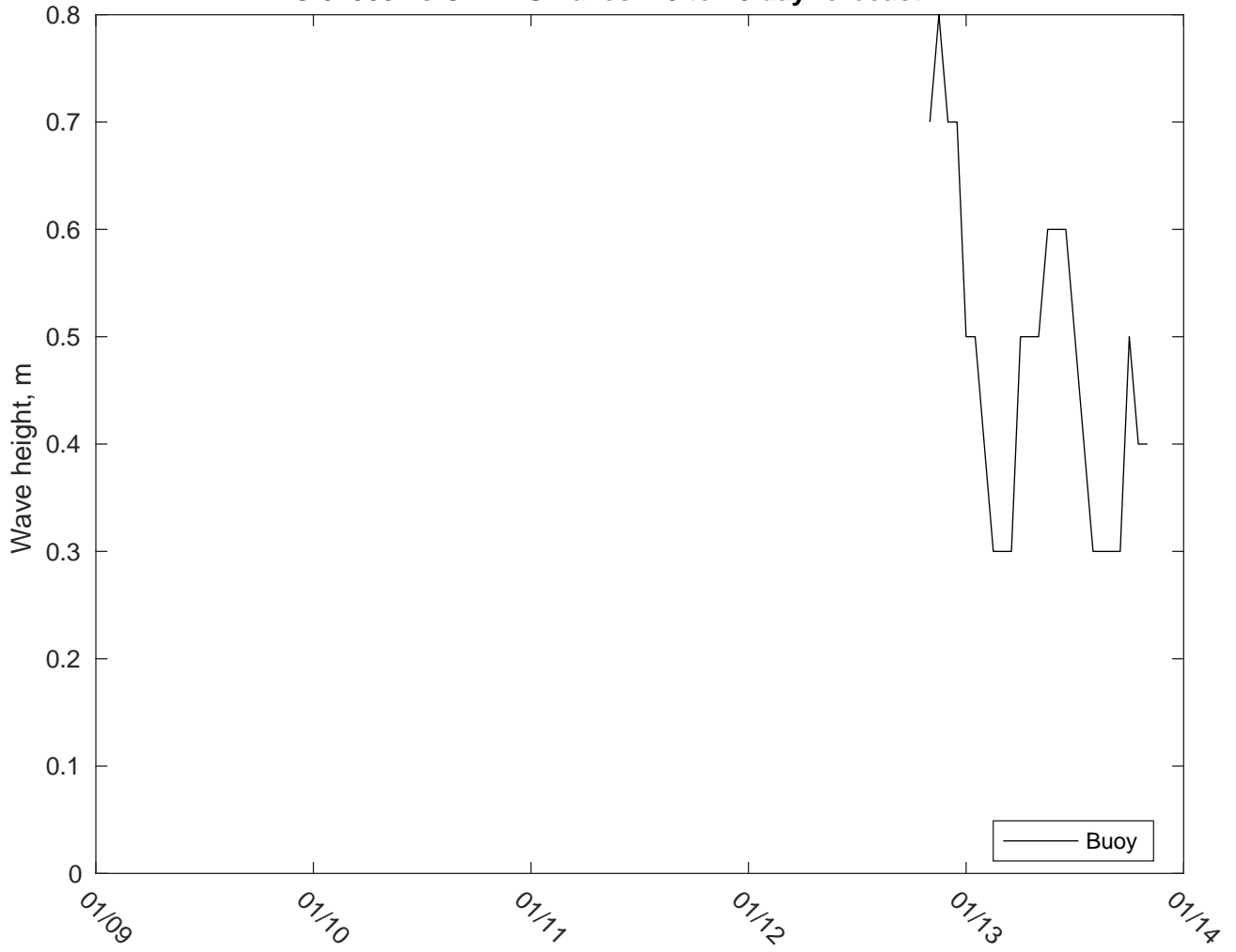
NDBC 62305 vs CMEMSWaves: 10 to 16 day forecast
