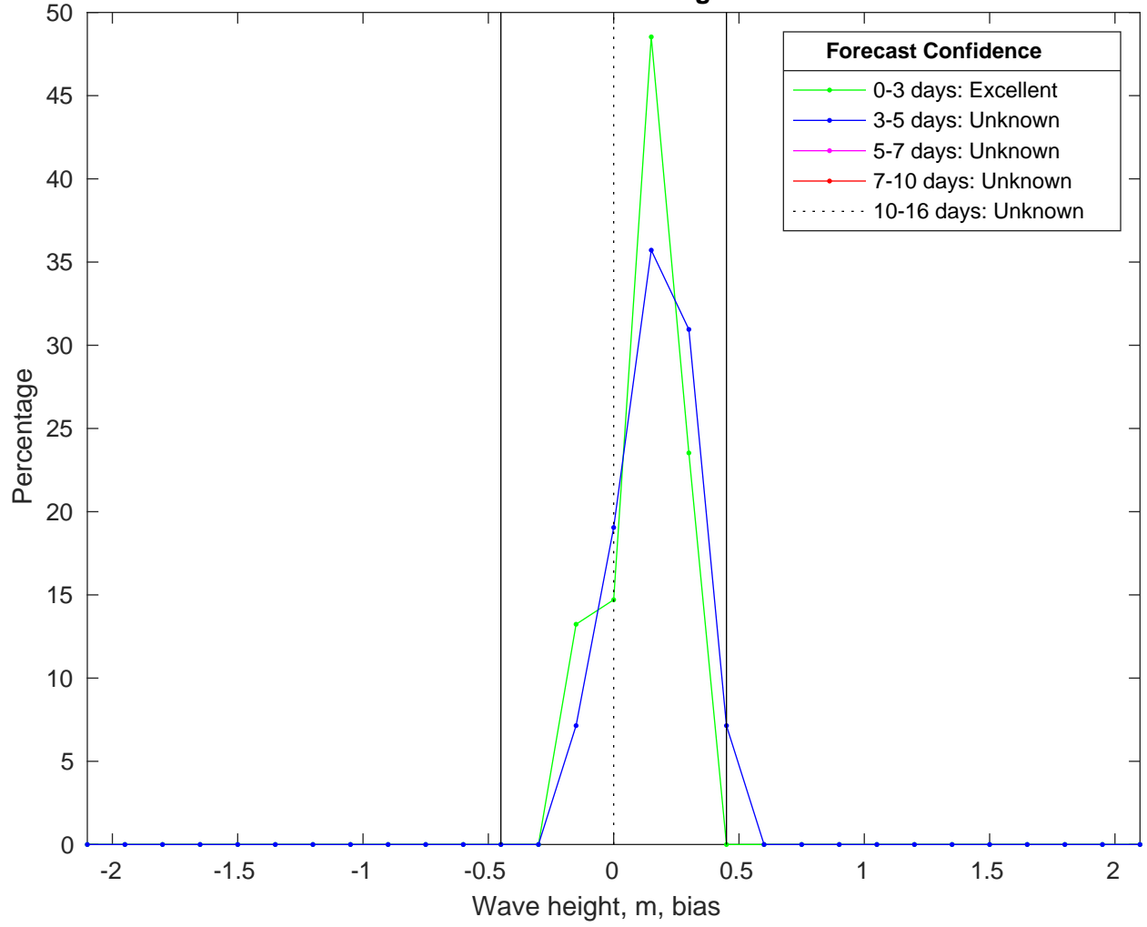
NDBC 62305 vs CMEMSWaves Bias Histogram: 13-Jan-2025
