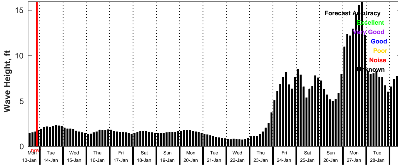
GFS Wave Forecast for NDBC 62305 from 13-Jan-2025 12:00:00 to 29-Jan-2025 12:00:00
