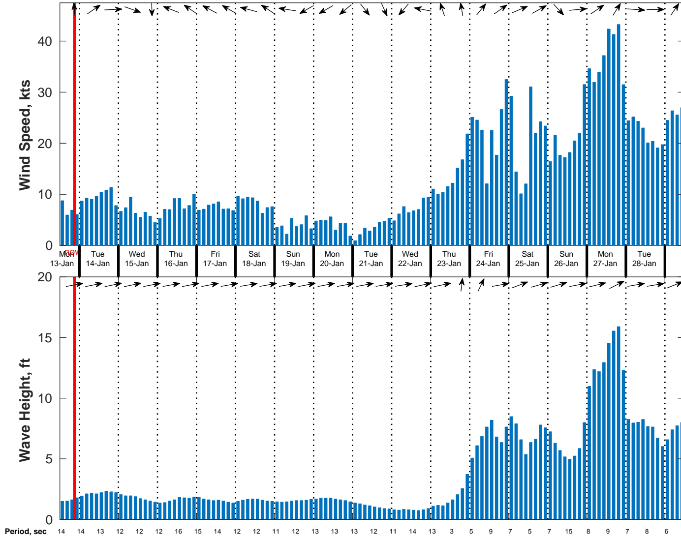
Wind & Wave Forecast for NDBC 62305 from 13-Jan-2025 12:00:00 to 29-Jan-2025 12:00:00
