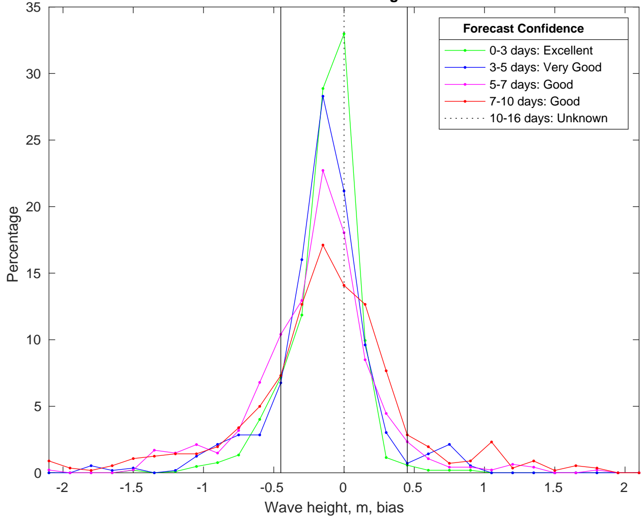
NDBC 41004 vs CMEMSWaves Bias Histogram: 15-Jan-2025
