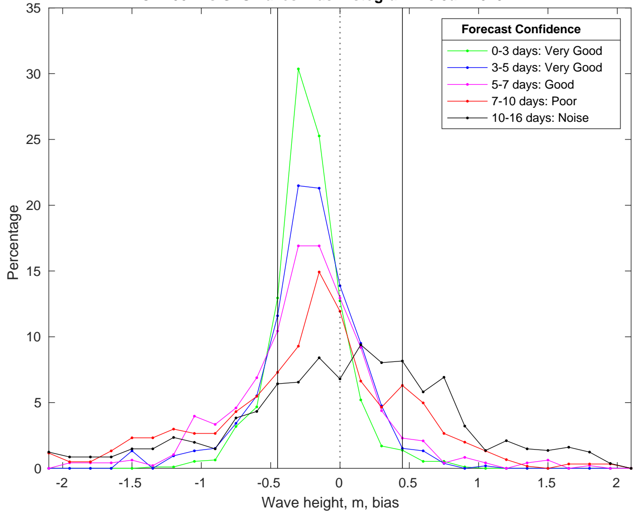
NDBC 41004 vs GFSWaves Bias Histogram: 15-Jan-2025
