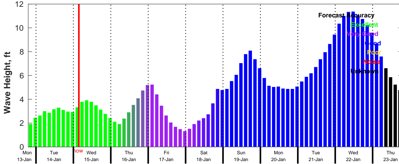
CMEMS Wave Forecast for NDBC 41004 from 13-Jan-2025 19:00:00 to 23-Jan-2025 19:00:00
