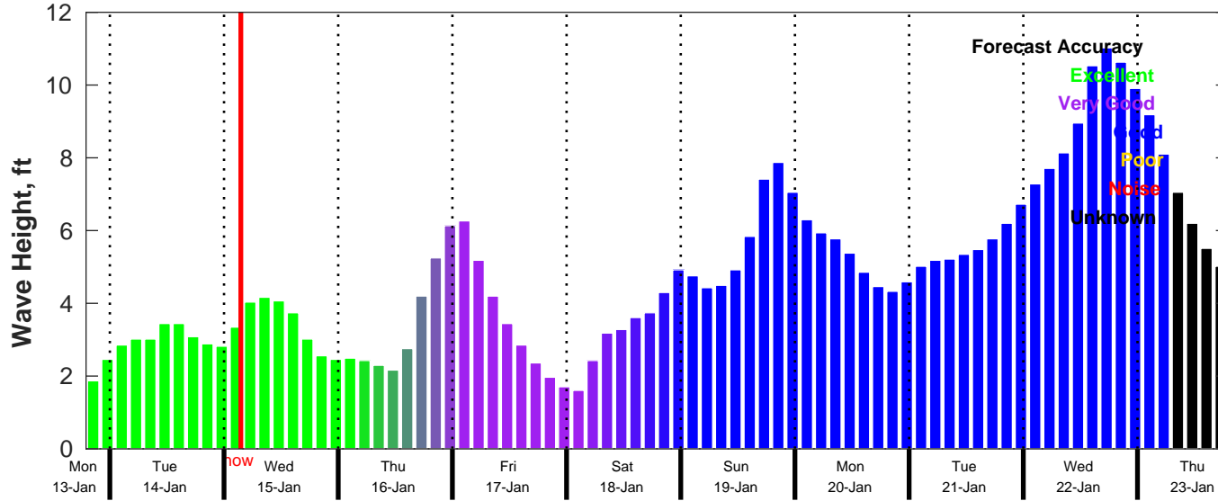
CMEMS Wave Forecast for NDBC 41013 from 13-Jan-2025 19:00:00 to 23-Jan-2025 19:00:00
