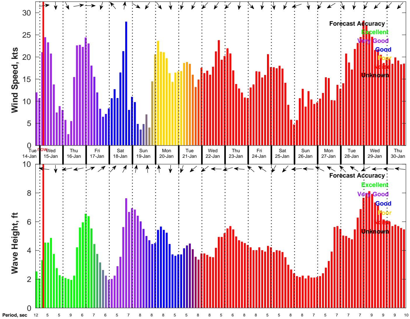
Wind & Wave Forecast for NDBC 41013 from 14-Jan-2025 19:00:00 to 30-Jan-2025 19:00:00
