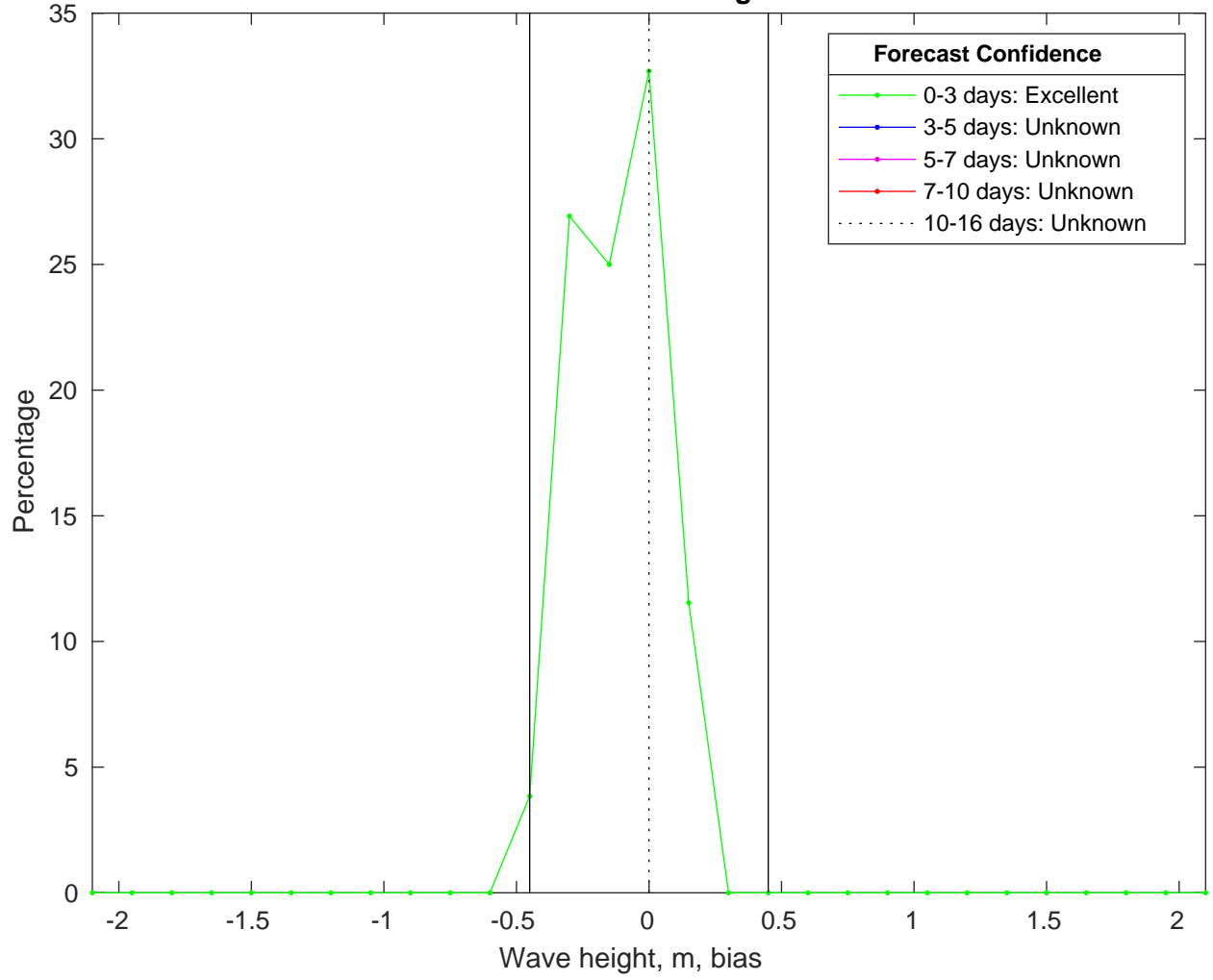
NDBC 41040 vs CMEMSWaves Bias Histogram: 15-Jan-2025
