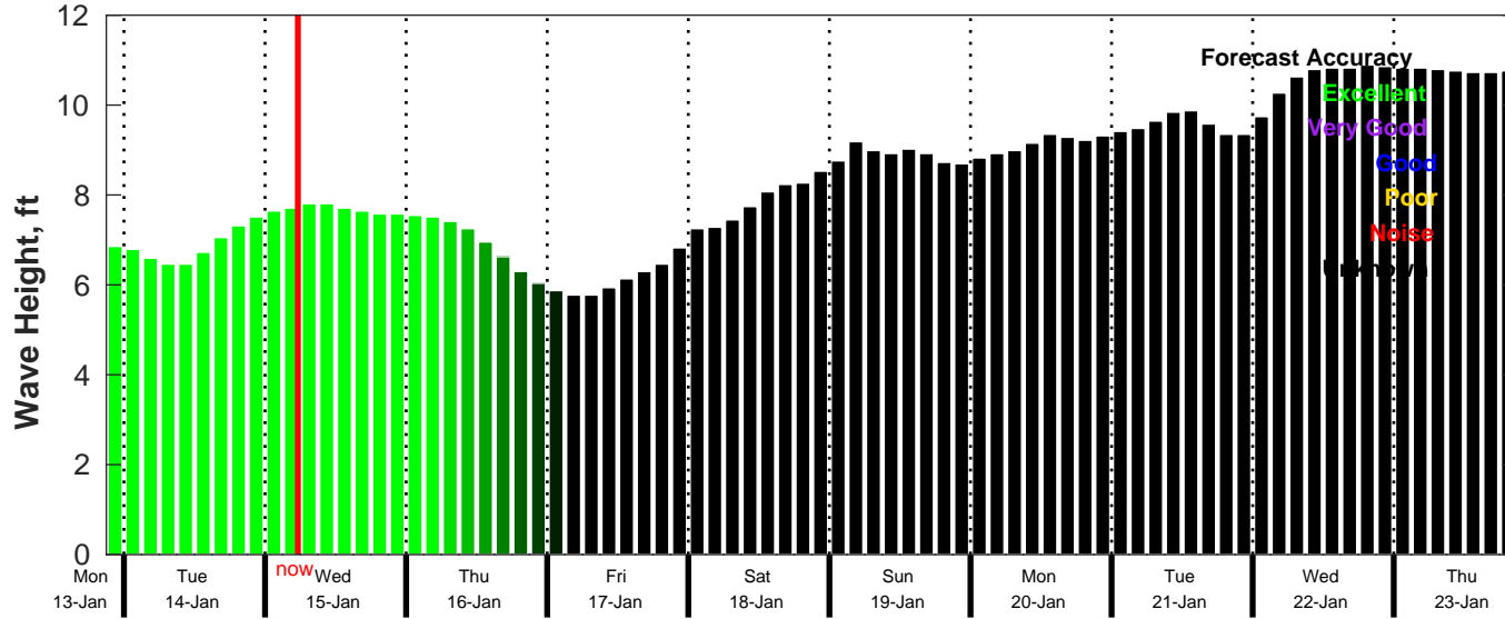
CMEMS Wave Forecast for NDBC 41040 from 13-Jan-2025 21:00:00 to 23-Jan-2025 21:00:00
