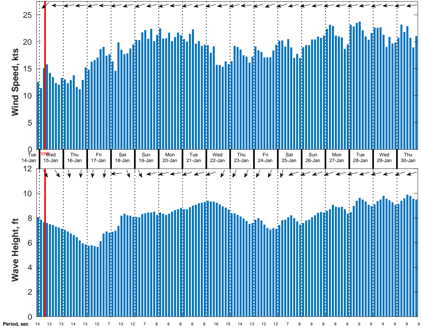
Wind & Wave Forecast for NDBC 41040 from 14-Jan-2025 21:00:00 to 30-Jan-2025 21:00:00
