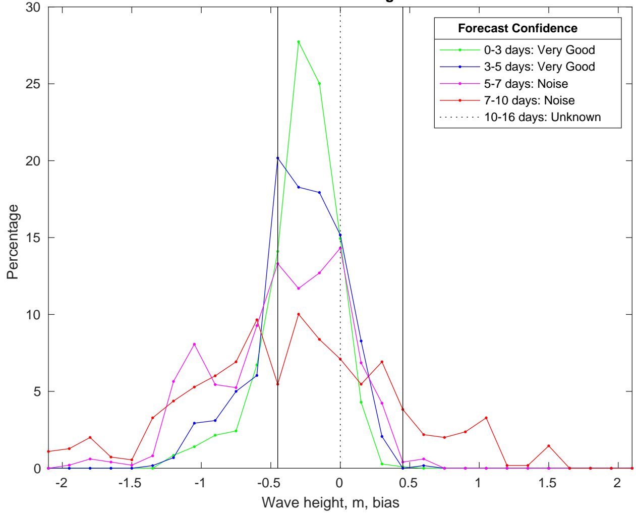
NDBC 42019 vs CMEMSWaves Bias Histogram: 15-Jan-2025
