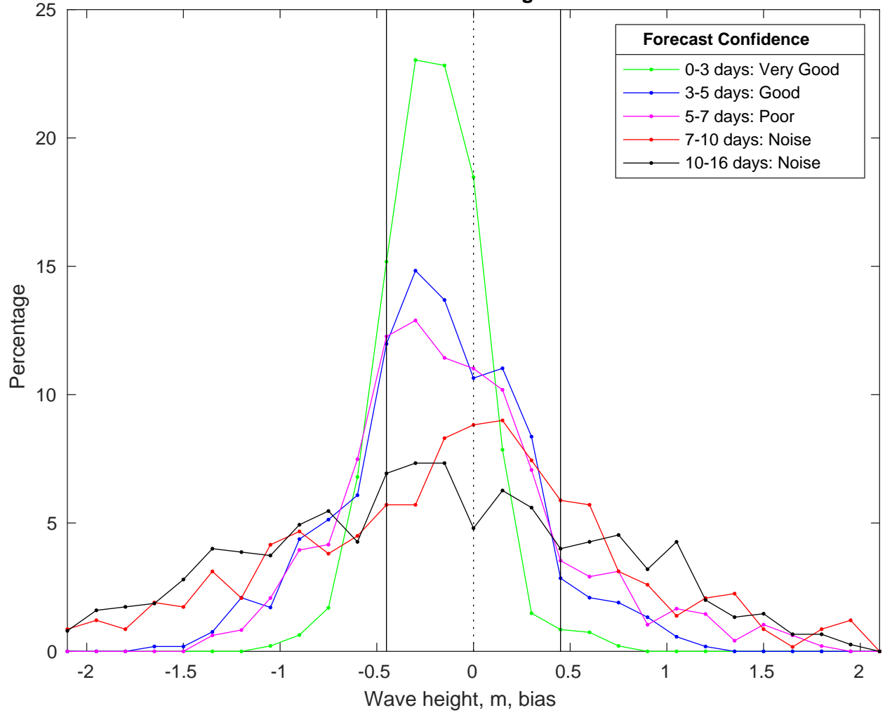
NDBC 42019 vs GFSWaves Bias Histogram: 15-Jan-2025
