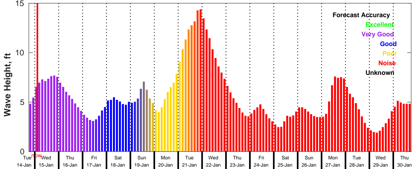
GFS Wave Forecast for NDBC 42019 from 14-Jan-2025 18:00:00 to 30-Jan-2025 18:00:00
