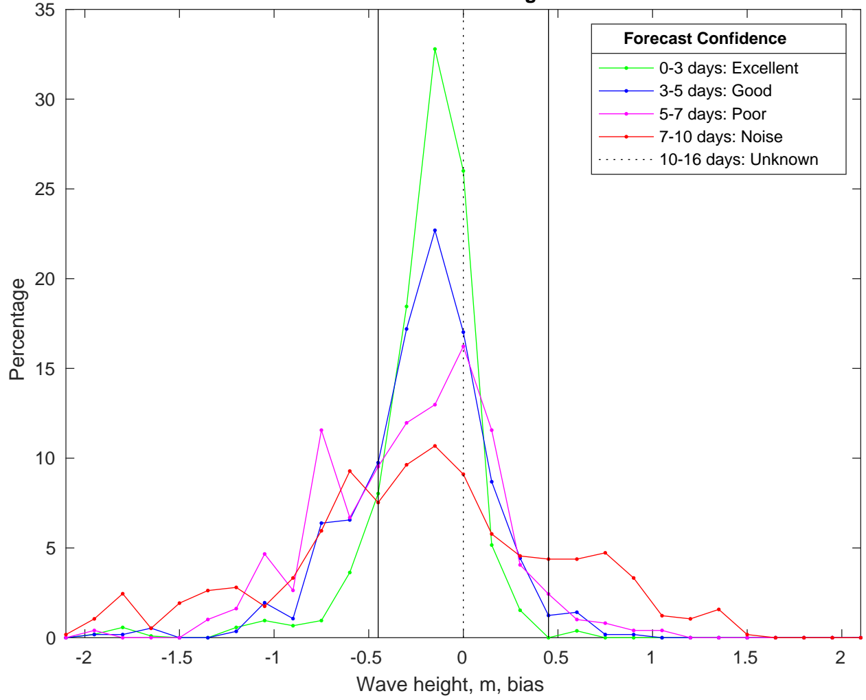
NDBC 42020 vs CMEMSWaves Bias Histogram: 15-Jan-2025
