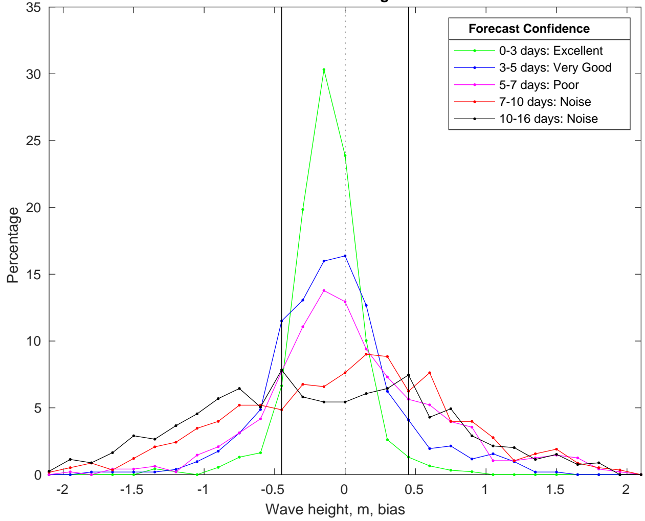
NDBC 42020 vs GFSWaves Bias Histogram: 15-Jan-2025
