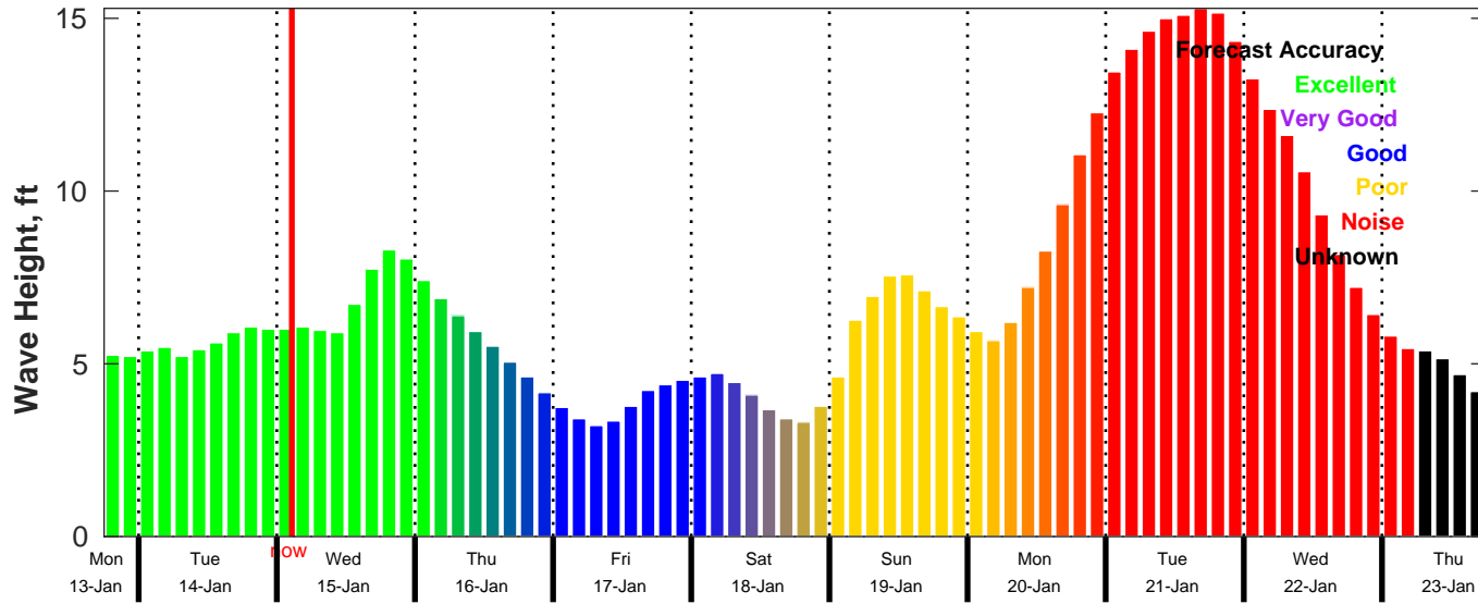
CMEMS Wave Forecast for NDBC 42020 from 13-Jan-2025 18:00:00 to 23-Jan-2025 18:00:00
