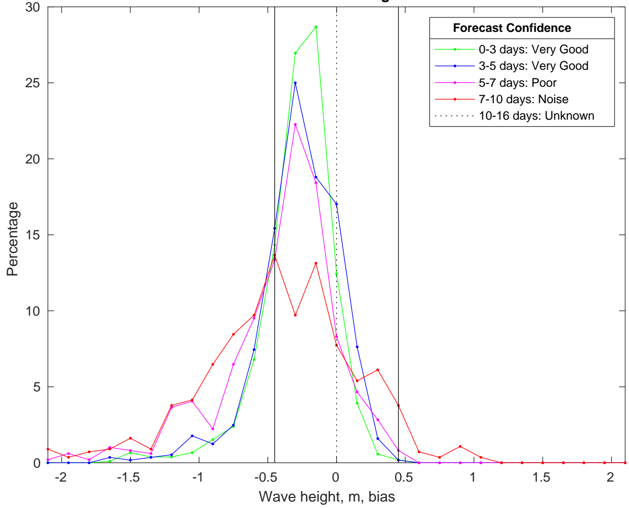
NDBC 42035 vs CMEMSWaves Bias Histogram: 15-Jan-2025
