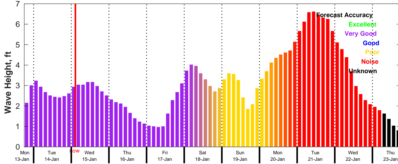
CMEMS Wave Forecast for NDBC 42035 from 13-Jan-2025 18:00:00 to 23-Jan-2025 18:00:00
