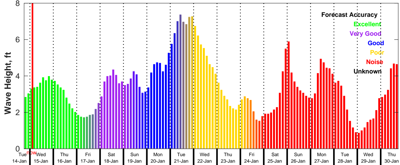
GFS Wave Forecast for NDBC 42035 from 14-Jan-2025 18:00:00 to 30-Jan-2025 18:00:00
