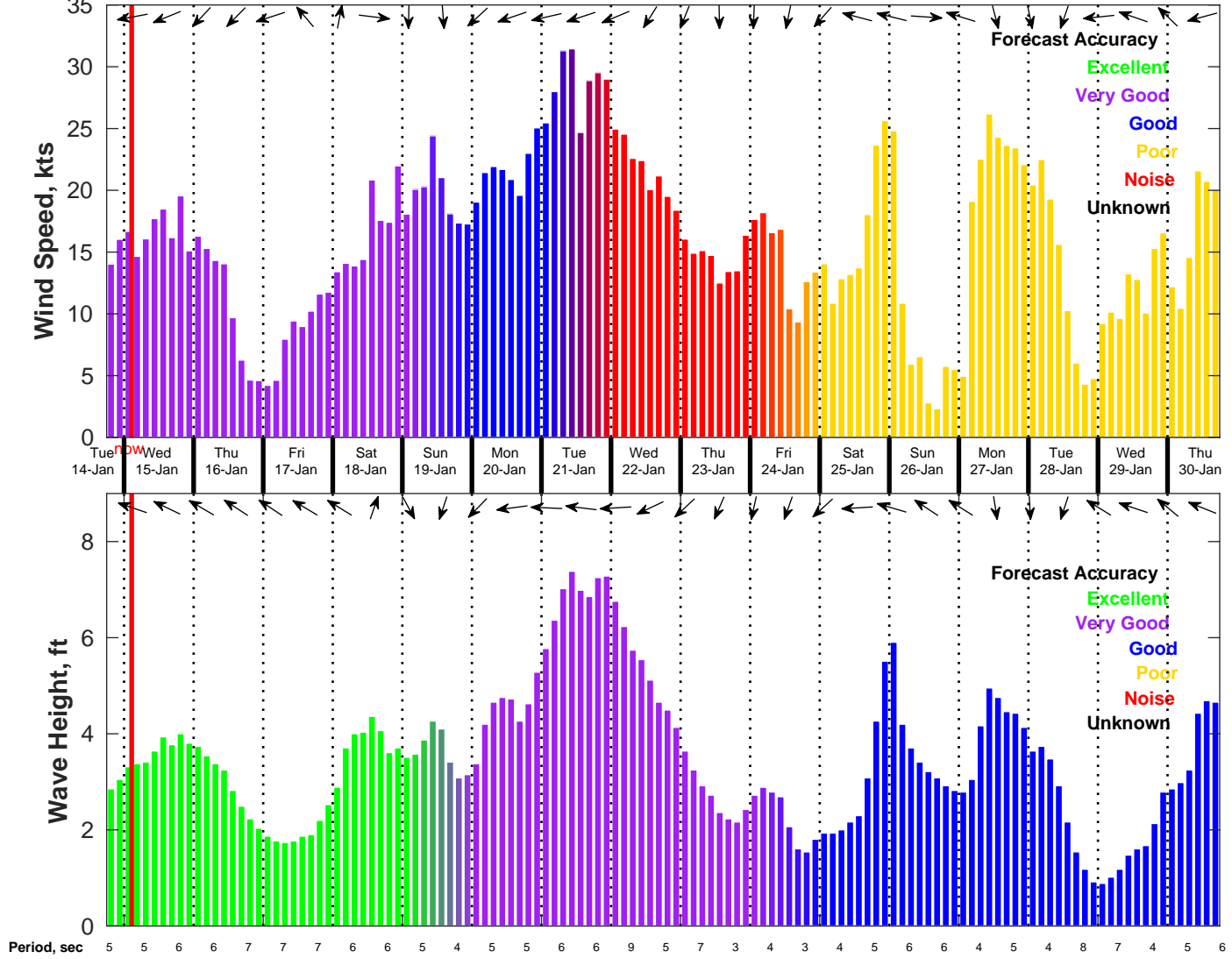
Wind & Wave Forecast for NDBC 42035 from 14-Jan-2025 18:00:00 to 30-Jan-2025 18:00:00
