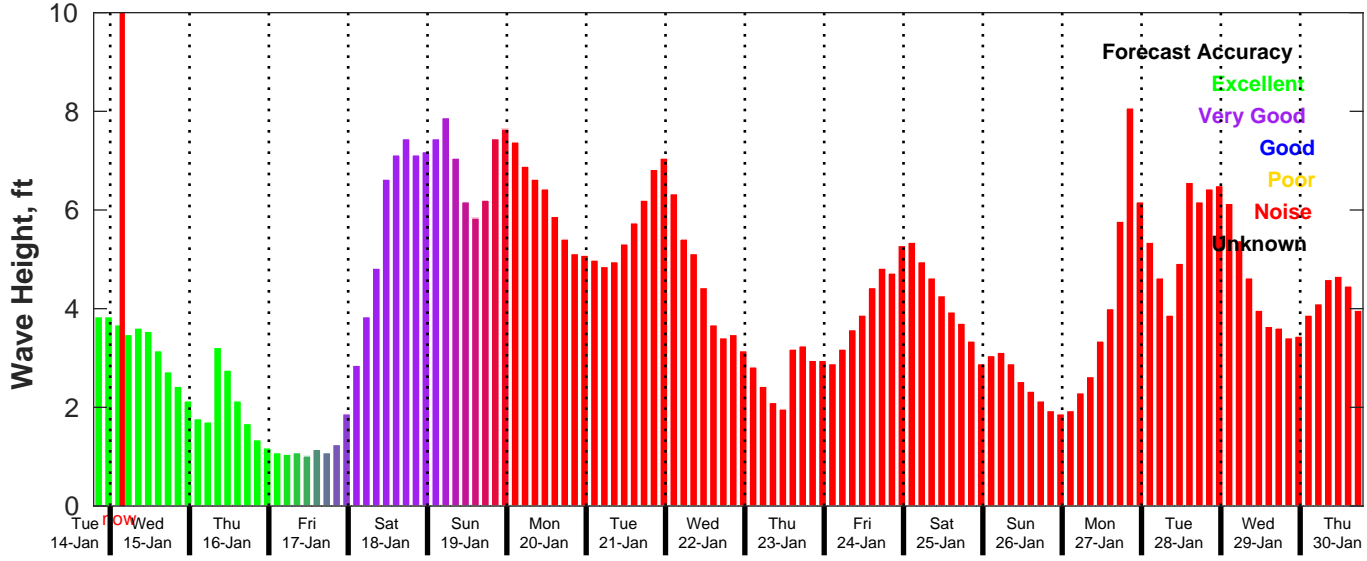
GFS Wave Forecast for NDBC 42036 from 14-Jan-2025 19:00:00 to 30-Jan-2025 19:00:00
