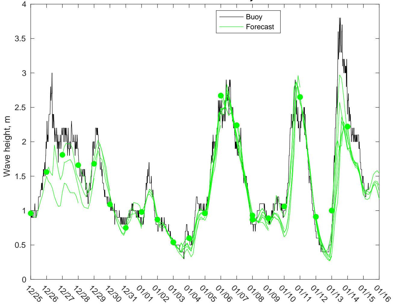
NDBC 42040 vs CMEMSWaves: 0 to 3 day forecast
