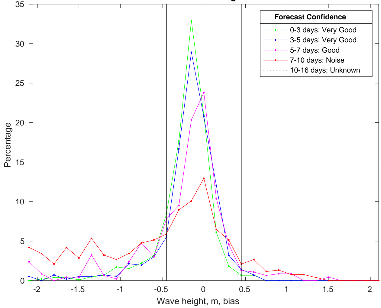
NDBC 42040 vs CMEMSWaves Bias Histogram: 15-Jan-2025
