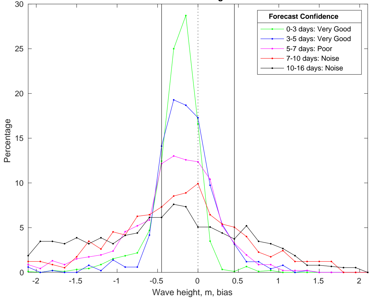
NDBC 42040 vs GFSWaves Bias Histogram: 15-Jan-2025
