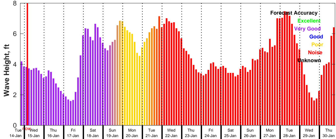
GFS Wave Forecast for NDBC 42040 from 14-Jan-2025 19:00:00 to 30-Jan-2025 19:00:00
