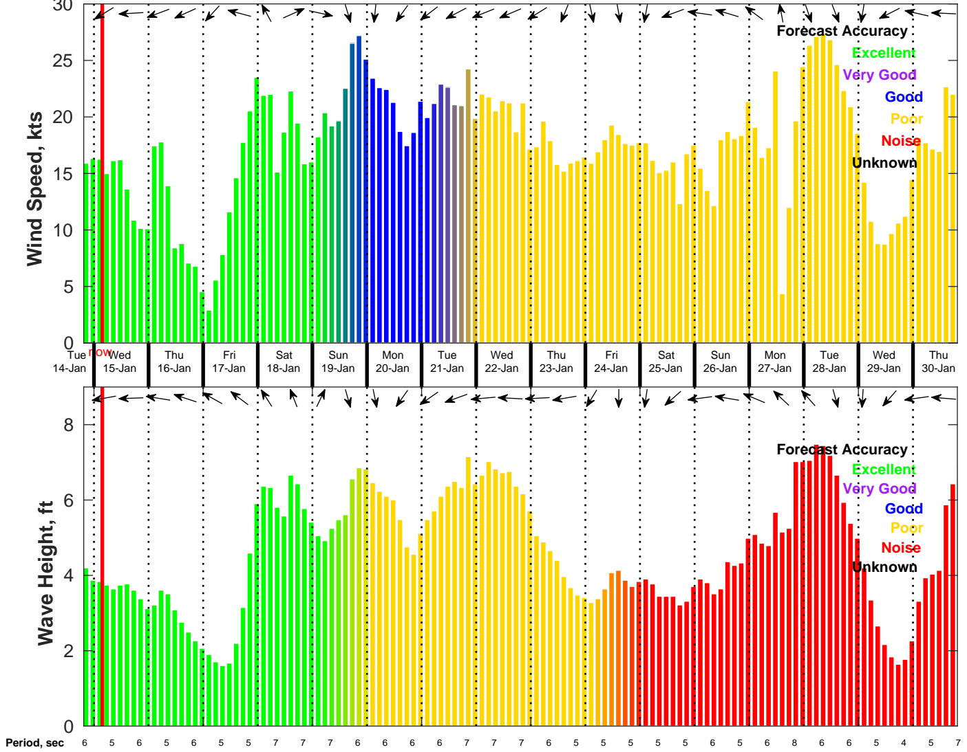
Wind & Wave Forecast for NDBC 42040 from 14-Jan-2025 19:00:00 to 30-Jan-2025 19:00:00
