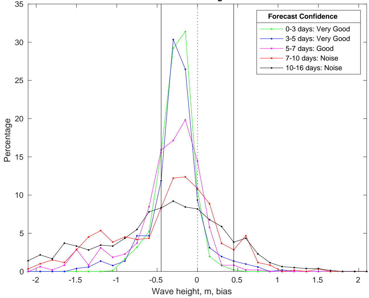
NDBC 42084 vs GFSWaves Bias Histogram: 15-Jan-2025
