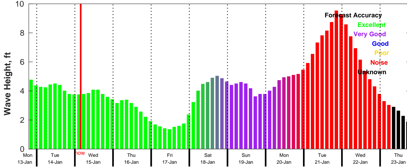
CMEMS Wave Forecast for NDBC 42084 from 13-Jan-2025 19:00:00 to 23-Jan-2025 19:00:00
