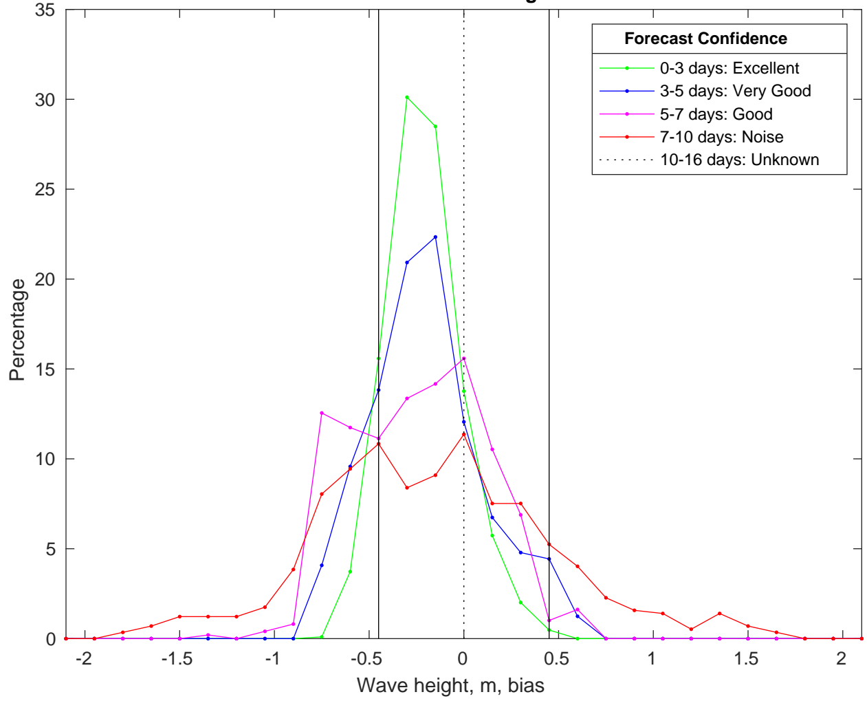
NDBC 42092 vs CMEMSWaves Bias Histogram: 15-Jan-2025
