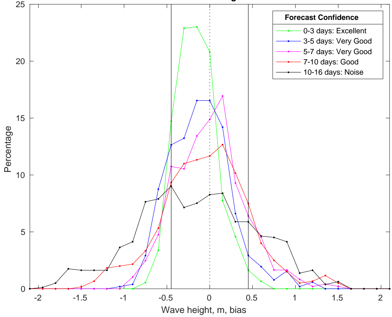
NDBC 42092 vs GFSWaves Bias Histogram: 15-Jan-2025
