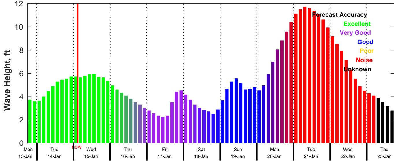
CMEMS Wave Forecast for NDBC 42092 from 13-Jan-2025 18:00:00 to 23-Jan-2025 18:00:00
