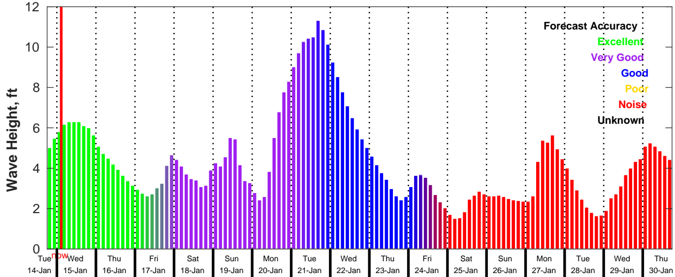
GFS Wave Forecast for NDBC 42092 from 14-Jan-2025 18:00:00 to 30-Jan-2025 18:00:00
