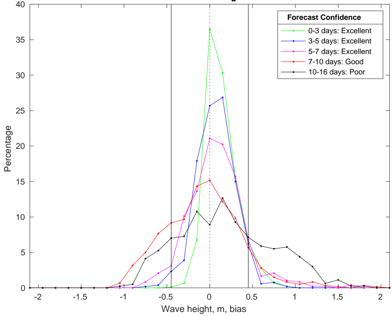
NDBC 44020 vs GFSWaves Bias Histogram: 15-Jan-2025
