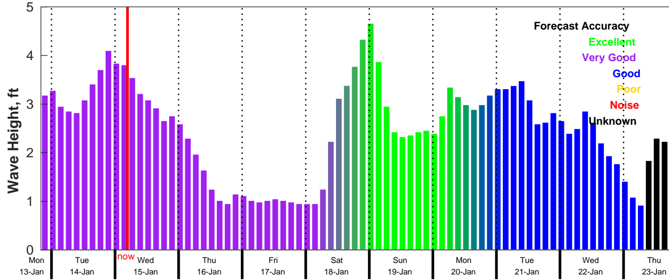
CMEMS Wave Forecast for NDBC 44020 from 13-Jan-2025 20:00:00 to 23-Jan-2025 20:00:00
