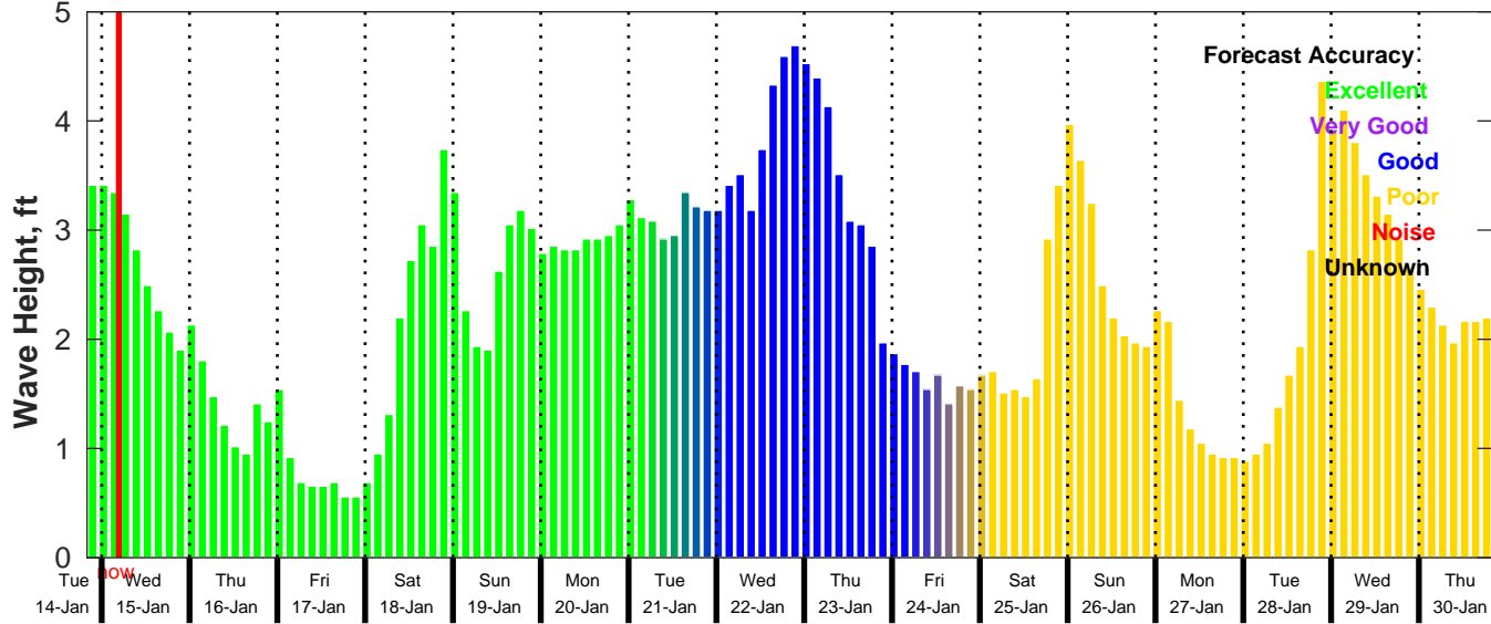
GFS Wave Forecast for NDBC 44020 from 14-Jan-2025 20:00:00 to 30-Jan-2025 20:00:00
