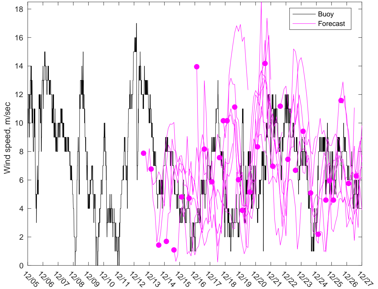
NDBC 44020 vs GFSWinds: 7 to 10 day forecast
