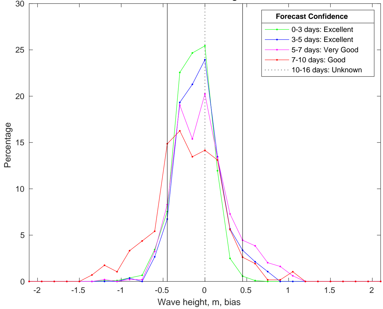
NDBC 46011 vs CMEMSWaves Bias Histogram: 15-Jan-2025
