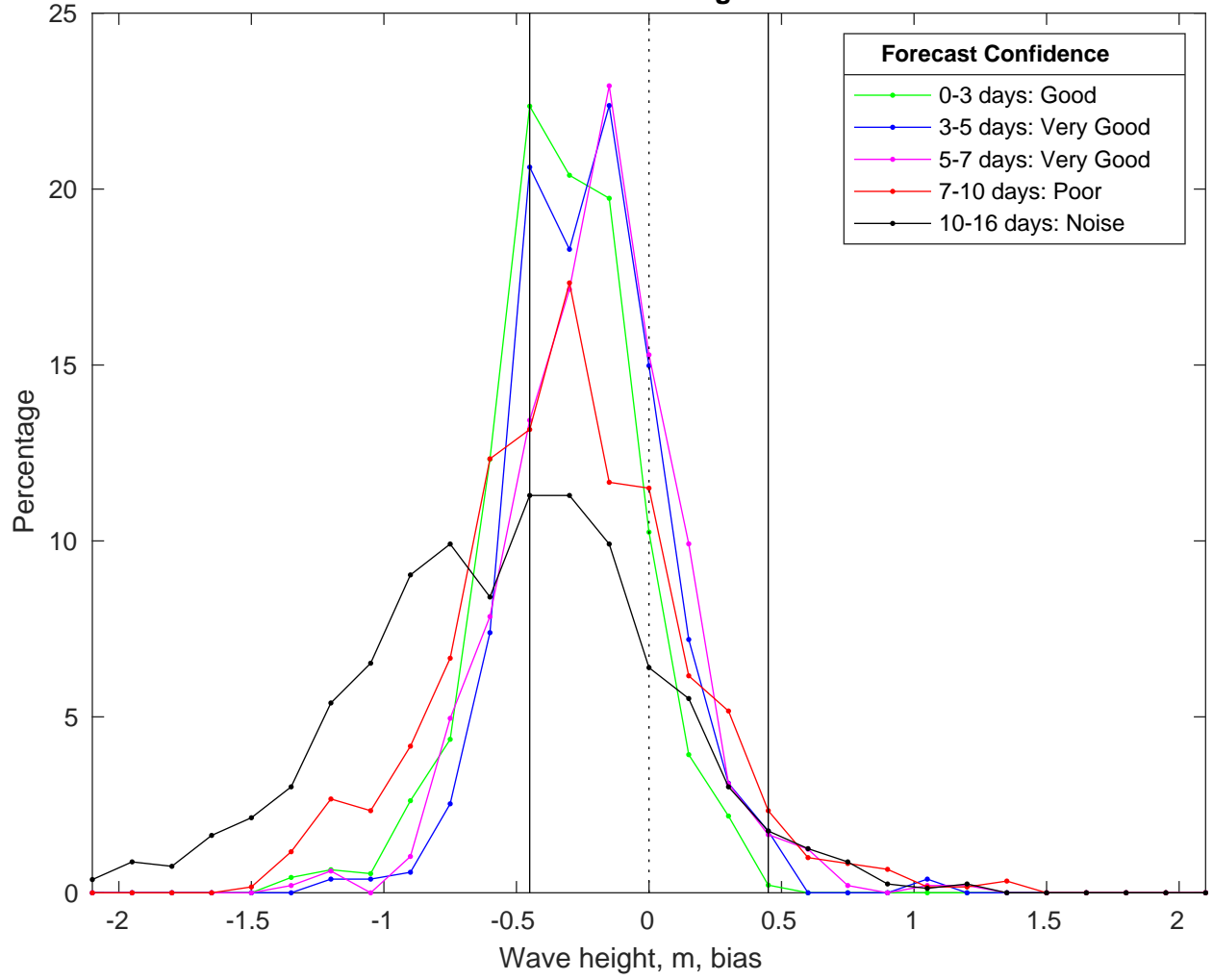
NDBC 46011 vs GFSWaves Bias Histogram: 15-Jan-2025
