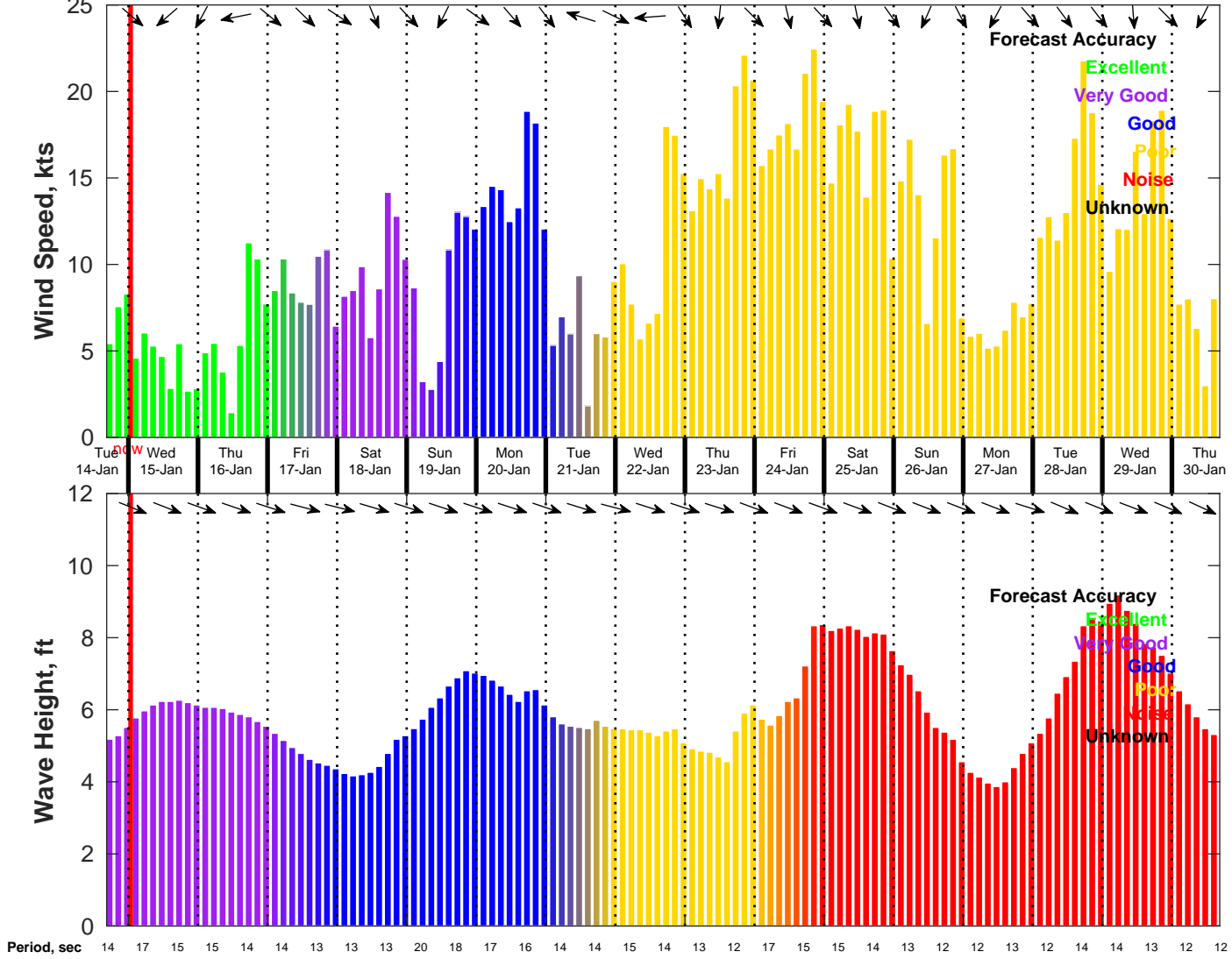
Wind & Wave Forecast for NDBC 46011 from 14-Jan-2025 16:00:00 to 30-Jan-2025 16:00:00
