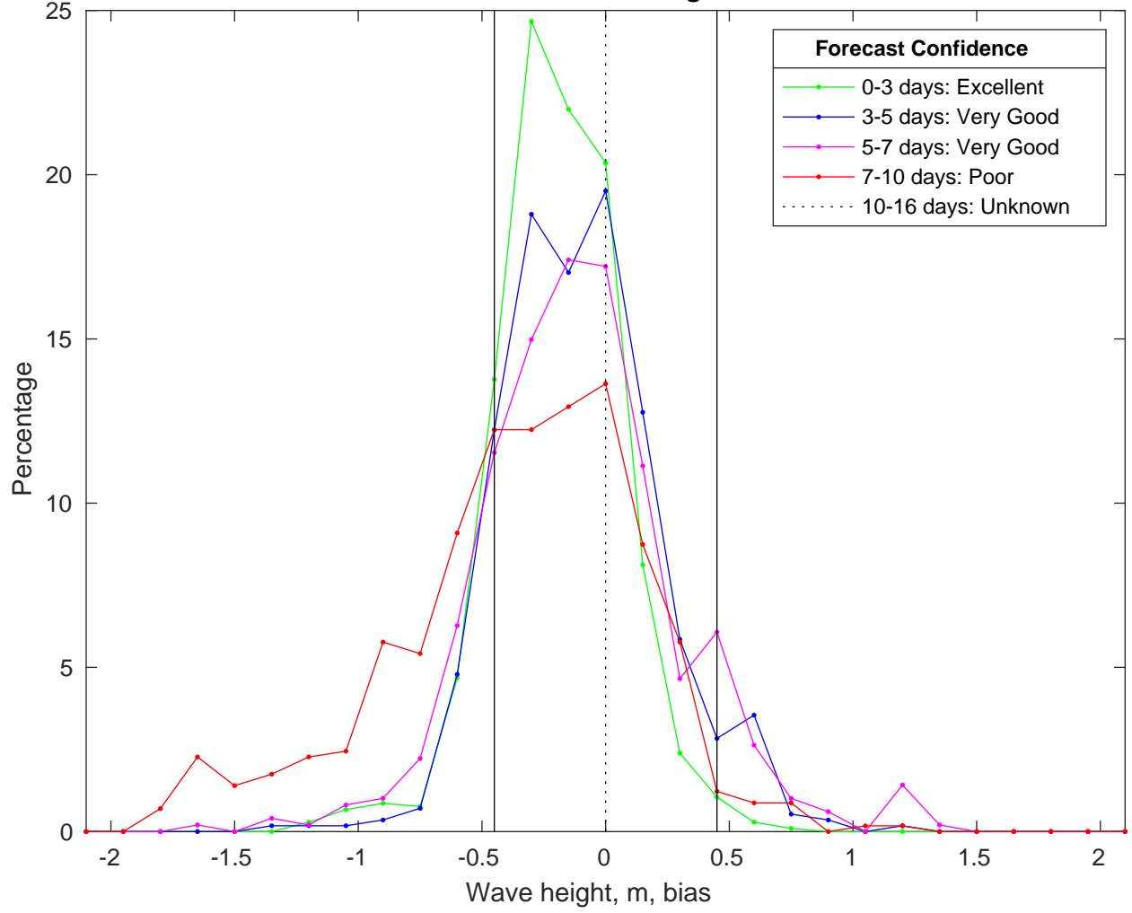
NDBC 46028 vs CMEMSWaves Bias Histogram: 15-Jan-2025
